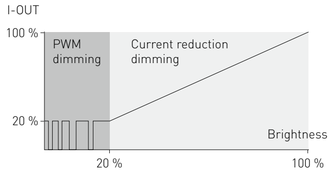
Hybrid dimming technique
