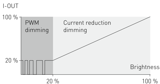
Hybrid dimming technique
